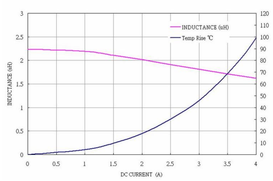
MLV-FY12N2R2N-M3
