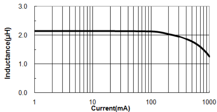
Inductance-Current Characteristics (Typ.)
