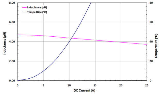
MMD-12CE-4R7M-V1
