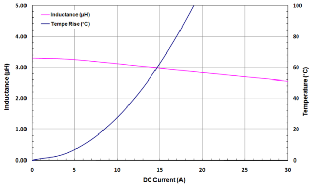
MMD-12CE-3R3M-V1
