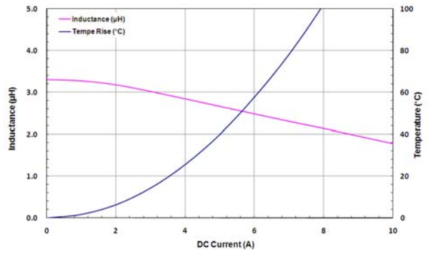
MAC105CZ-3R3M-M2
