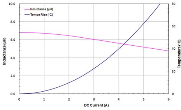
MAC106BD-6R8M-X2
