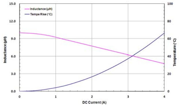
MAC106BD-100M-X2
