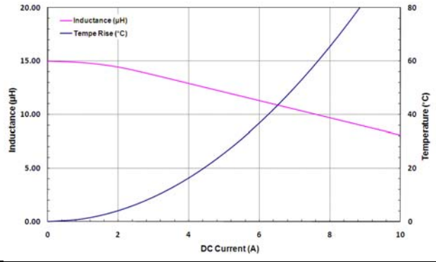
MAC110DZ-150M-M1
