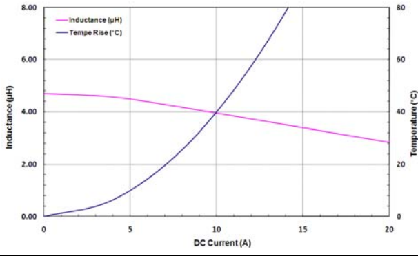
MAC110DZ-4R7M-M1
